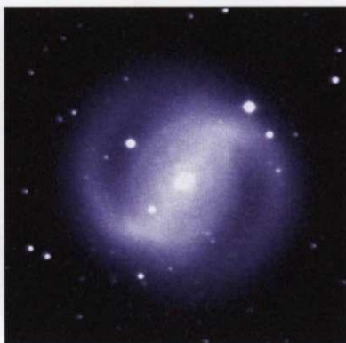
Spiral bar galaxy NGC 4314
