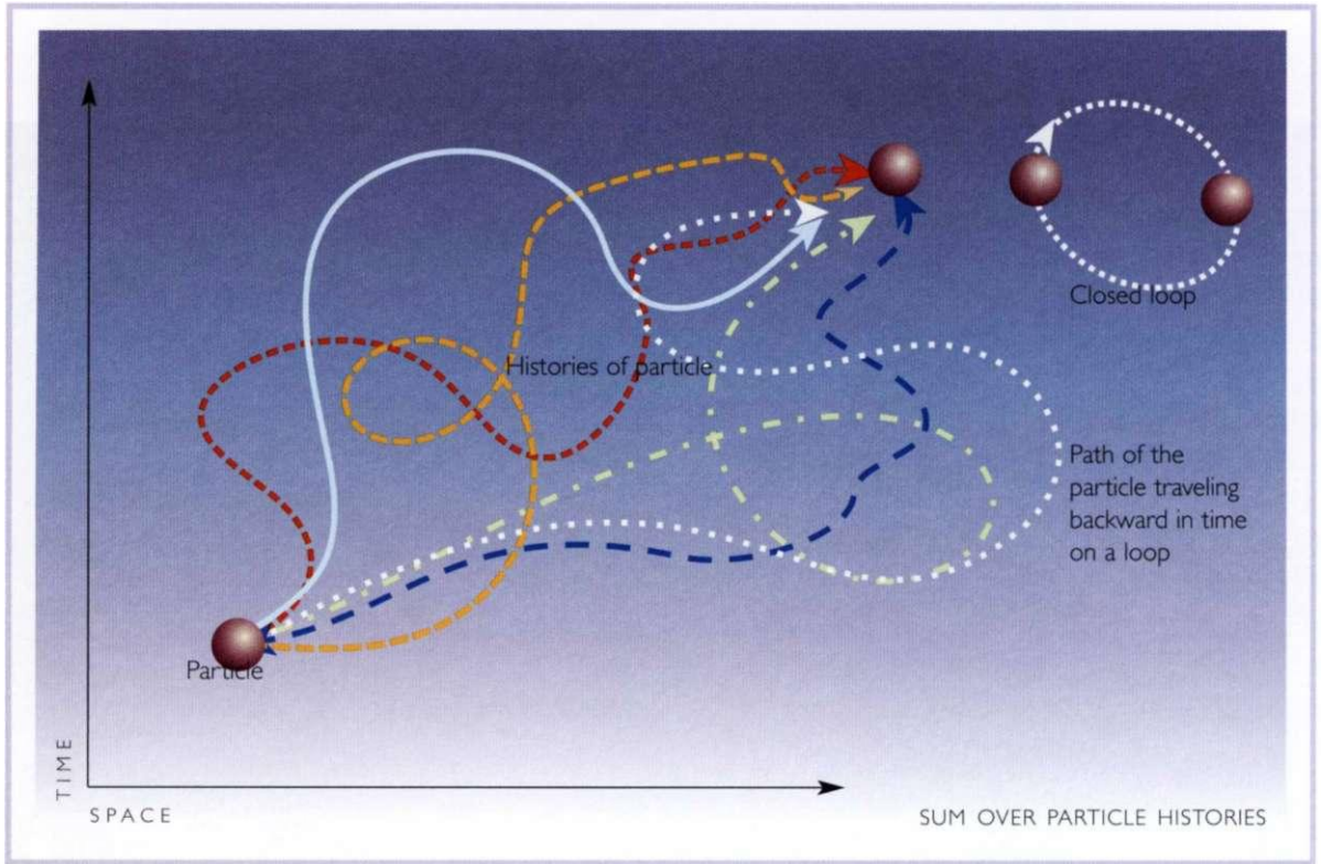
(FIG. 5.13) The Feynman sum over histories has to include histories in which particles travel back in time, and even histories that are closed loops in time and space.
