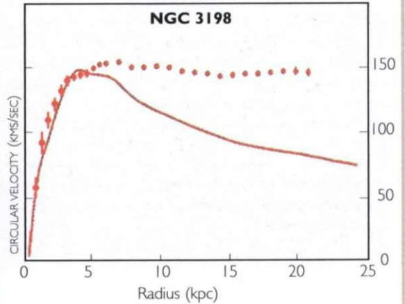
ROTATION CURVE FOR SPIRAL GALAXY NGC 3198
