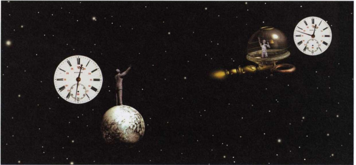
(FIG. 4.6) In the flat spacetime of special relativity observers moving at different speeds will have different measures of time, but we can use the Schrodinger equation in any of these times to predict what the wave function will be in the future.
