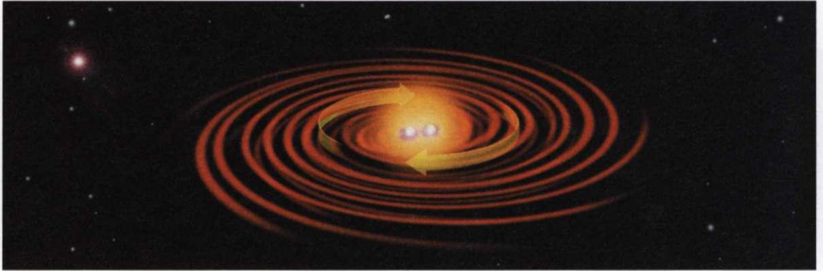
Two compact neutron stars spiraling in toward one another
