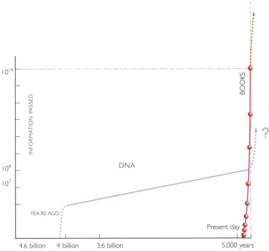
The development of complexity since the formation of the Earth (not to scale).
